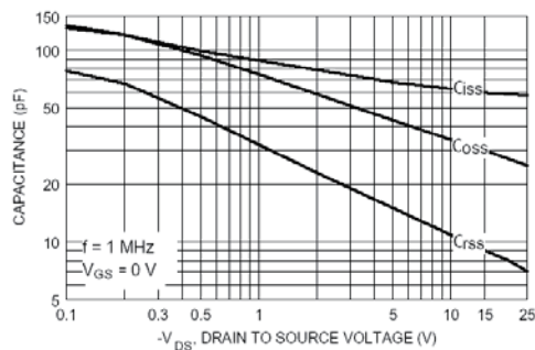
Figure 19. Capacitance Characteristics.
