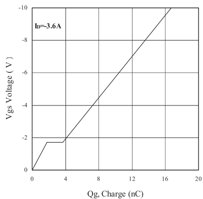
Figure 5. Gate Charge
