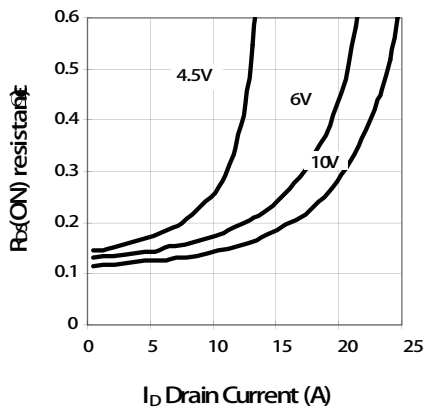
On-Resistance vs. Drain Current
