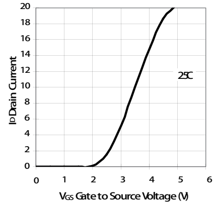
Transfer Characteristics
