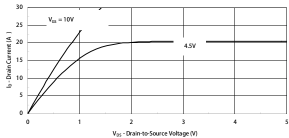
Output Characteristics
