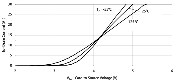
Transfer Characteristics
