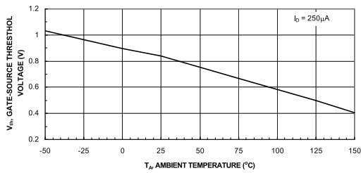
Figure 9. Threshold Voltage
