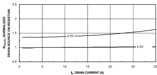
Figure 3. On-Resistance vs. Drain Current
