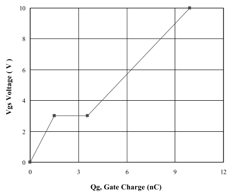
Figure 5. Gate Charge
