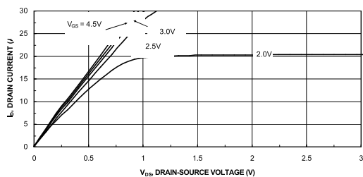
Figure 1. Output Characteristics
