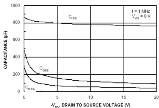
Figure 8. Capacitance Characteristic
