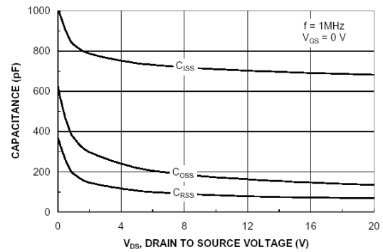
Figure 8. Capacitance Characteristic
