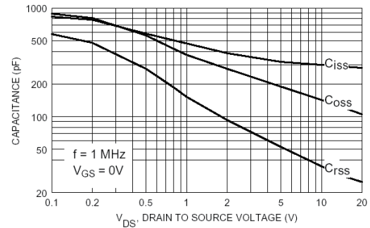
Figure 8. Capacitance Characteristics.
