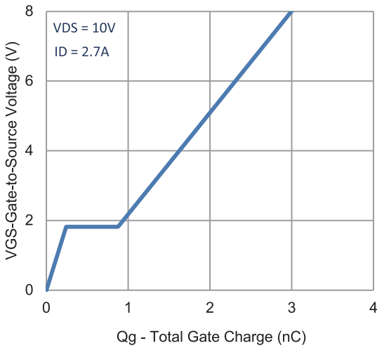
7. Gate Charge
