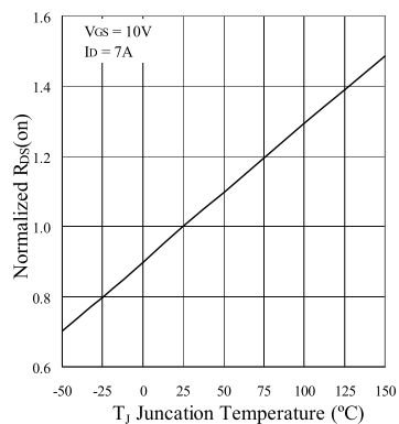
Figure 6. On-Resistance Variation with Temperature
