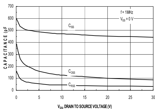
Figure 4. Capacitance Characteristics
