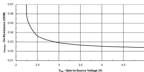
On-Resistance vs. Gate-to-Source Voltage
