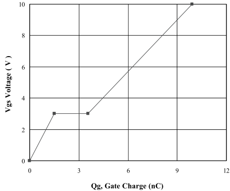
Figure 5. Gate Charge
