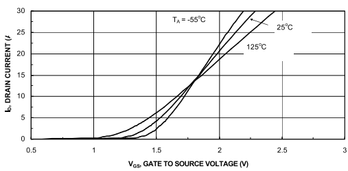
Figure 2. Transfer Characteristics
