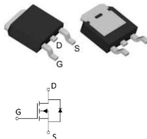
TO252
