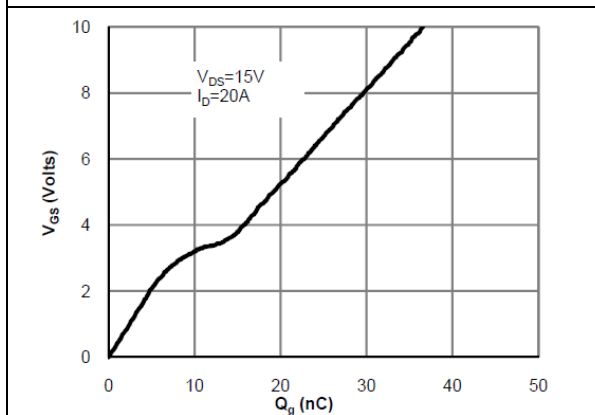
Figure 7. Gate-Charge Characteristics
