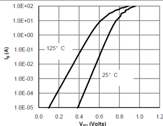
Figure 6. Body-Diode Characteristics
