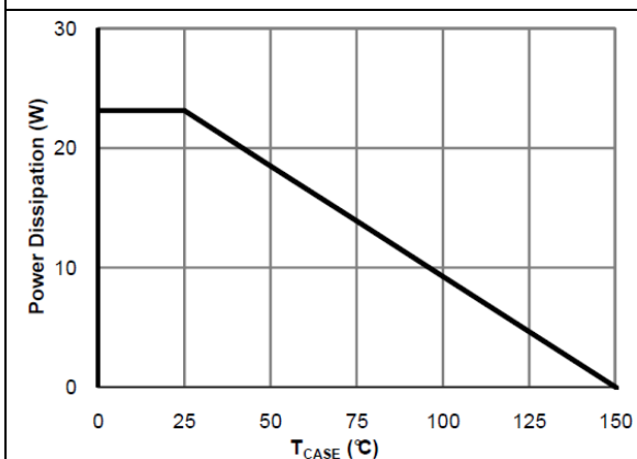
Figure 12. Power De-rating
