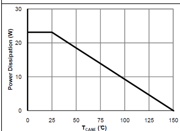
Figure 12. Power De-rating
