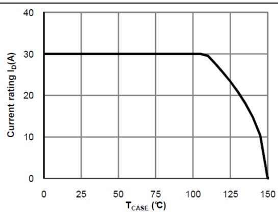
Figure 13. Current De-rating
