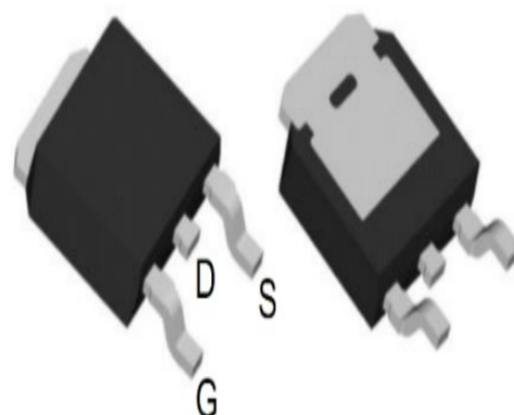
TO-252
