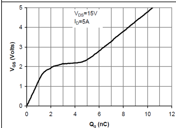
Figure 7. Gate-Charge Characteristics
