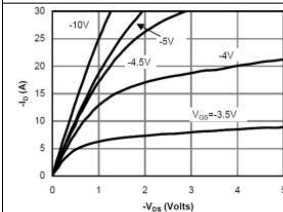
Figure 1. On-Regin Characteristics
