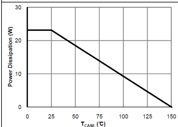
Figure 12. Power De-rating
