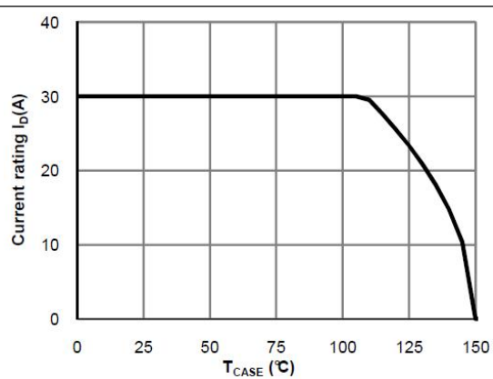
Figure 13. Current De-rating
