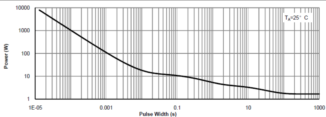
Figure 14. Single Pulse Power Rating Junction-to-Ambient
