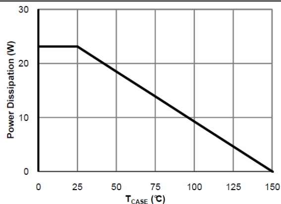
Figure 12. Power De-rating
