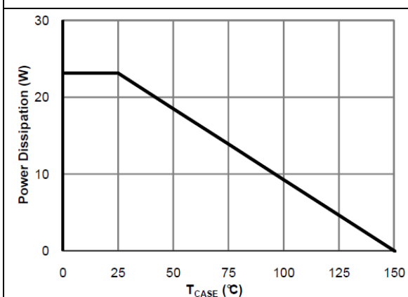
Figure 12. Power De-rating
