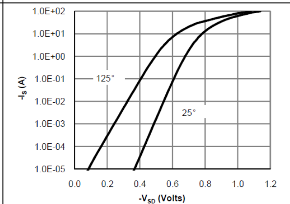
Figure 6. Body-Diode Characteristics
