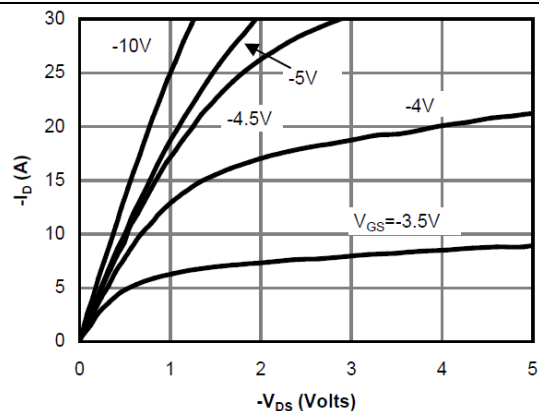
Figure 1. On-Regin Characteristics
